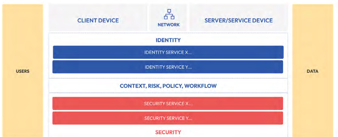
Figure 1: High-level Identity Defined Security Architecture
